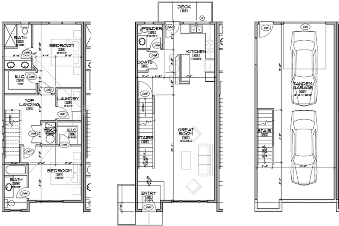
UPPER LEVEL FLOOR PLAN SCALE: 1/4" = 1'-0"
